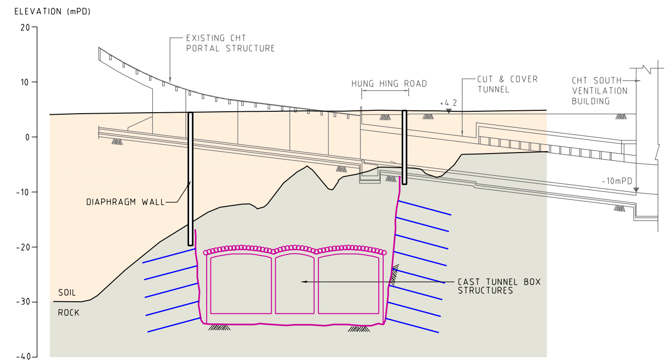
STAGE 2 : EXCAVATION OF ROCK BELOW TEMPORARY ROOF BY DRILLING AND ROCK BREAKING
